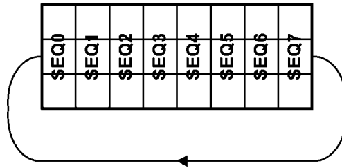
FIGURE 17. State Machine Generating Fixed Pattern Sequence
