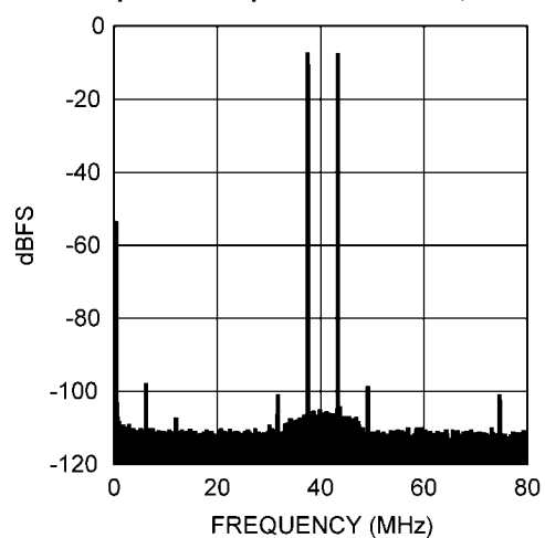
Two Tone Spectral Response @ 197 MHz, 203 MHz
