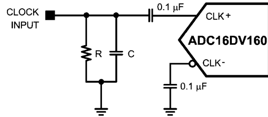
FIGURE 11. Singled-Ended 1.8V Clocking, Capacitive AC Coupled
