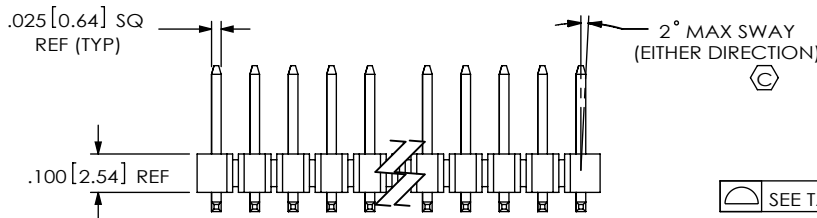
FIG 1 TSM-1XX-XX-XXX-DV SHOWN
