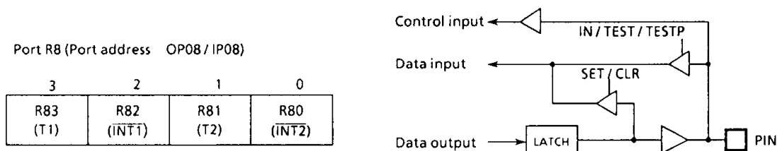
Figure 3-9. Port R8
