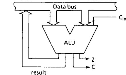
Figure 2-11. ALU
