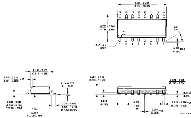
S.O. Package (M) Order Number DM74ALS109AM Package Number M16A
