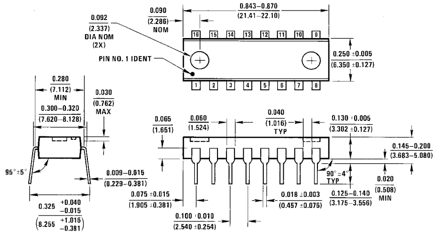
Molded Dual-In-Line Package (N) Order Number DM74ALS109AN Package Number N16A
