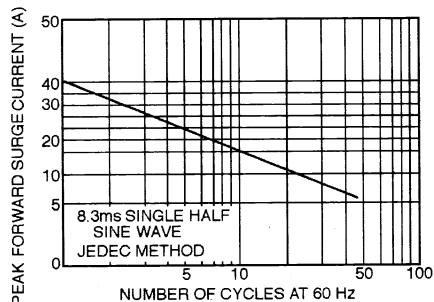
FIGURE 6 – MAXIMUM NON - REPETITIVE FORWARD SURGE CURRENT - UNIDIRECTIONAL ONLY
