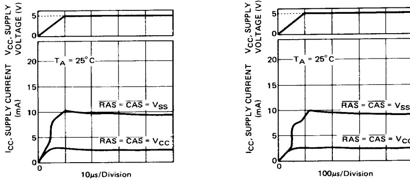
Fig. 21 — CURRENT WAVE FORM DURING POWER UP (ON MEMORY BOARD)
