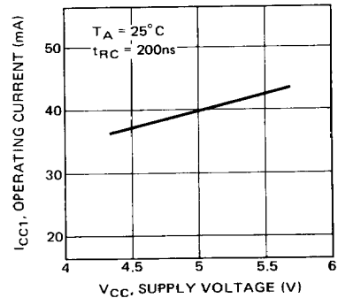
Fig. 6 — OPERATING CURRENT vs SUPPLY VOLTAGE
