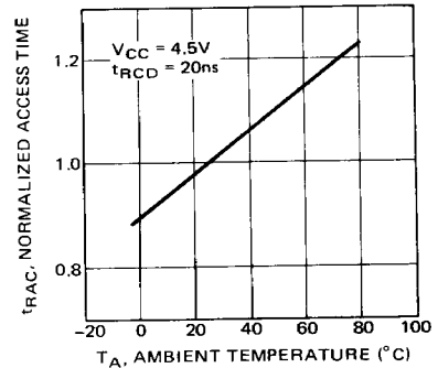
Fig. 4 — NORMALIZED ACCESS TIME vs AMBIENT TEMPERATURE
