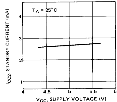
Fig. 8 — STANDBY CURRENT vs SUPPLY VOLTAGE
