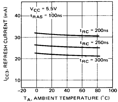
Fig. 12 — REFRESH CURRENT vs AMBIENT TEMPERATURE
