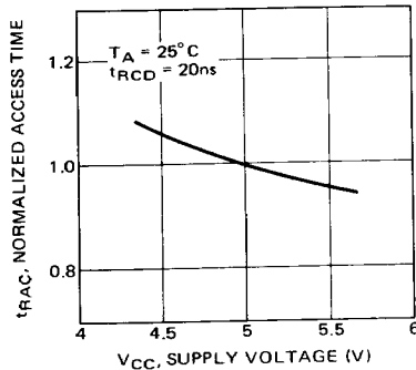
Fig. 3 — NORMALIZED ACCESS TIME vs SUPPLY VOLTAGE
