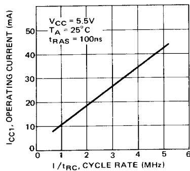
Fig. 5 — OPERATING CURRENT vs CYCLE RATE
