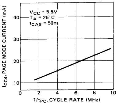
Fig. 13 — PAGE MODE CURRENT vs CYCLE RATE
