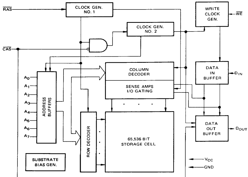
Fig. 1 – MB 8264A BLOCK DIAGRAM
