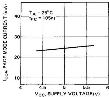
Fig. 14 — PAGE MODE CURRENT vs SUPPLY VOLTAGE
