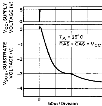
Fig. 22 — SUBSTRATE VOLTAGE vs SUPPLY VOLTAGE (DURING POWER UP)
