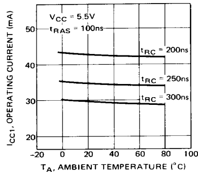
Fig. 7 — OPERATING CURRENT vs AMBIENT TEMPERATURE
