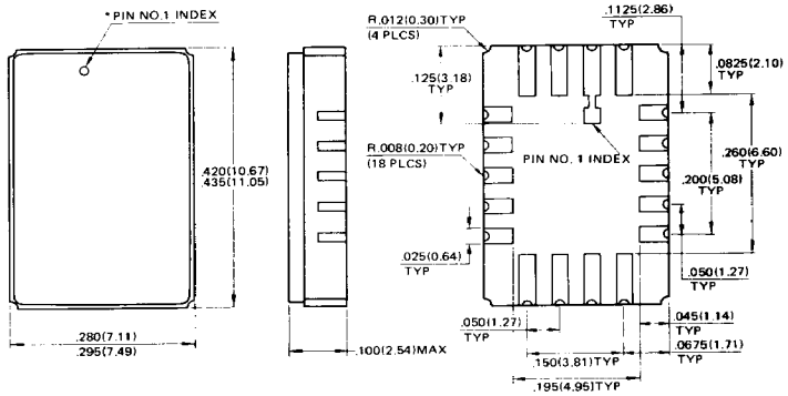
18-PAD CERAMIC (FRIT SEAL) LEADLESS CHIP CARRIER (CASE No.: LCC-18C-F02)
