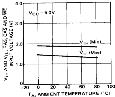
Fig. 19 — RAS, CAS AND WE VOLTAGE vs AMBIENT TEMPERATURE
