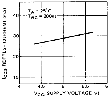
Fig. 11 — REFRESH CURRENT vs SUPPLY VOLTAGE
