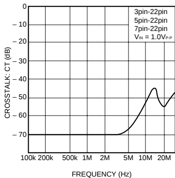
Fig. 14 Crosstalk characteristic (OUT1)
