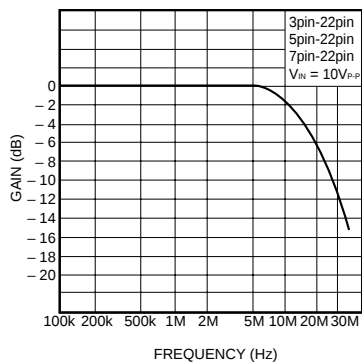
Fig. 13 Frequency characteristic(OUT1)
