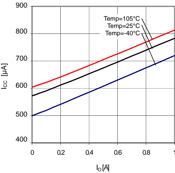
Figure 30. I_O-I_{CC}
