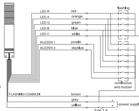
continuous and flashing light with alarm AC/DC 24V
