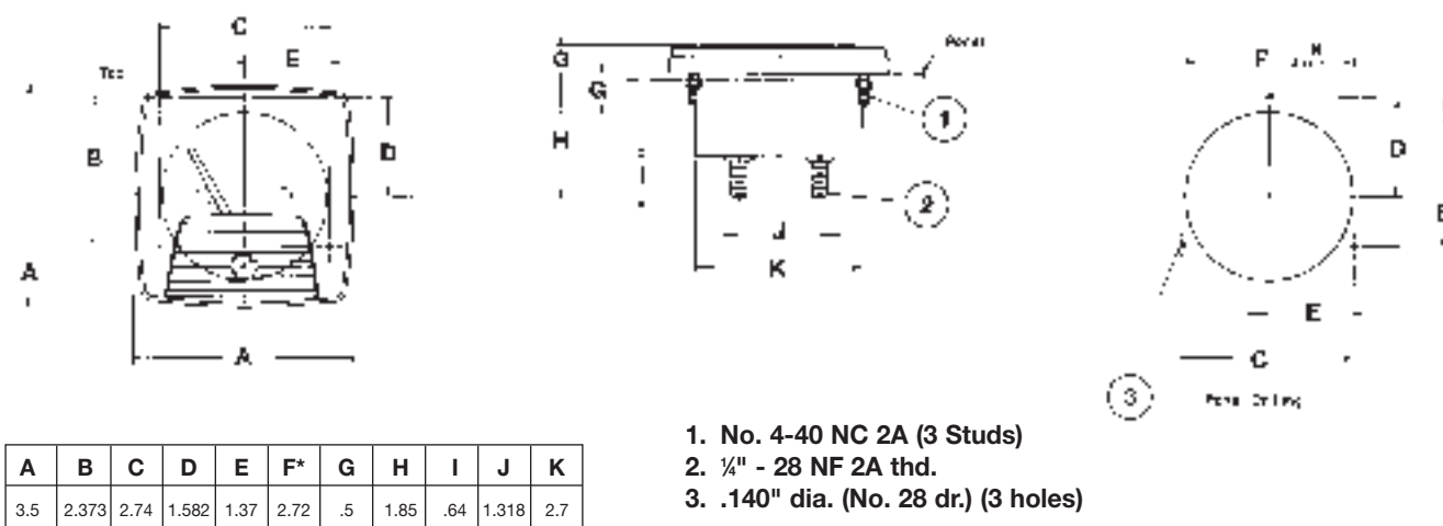
Fig. 3. New Big Look 3½-inch Types 250 & 254 *2.860 dia. with shield
