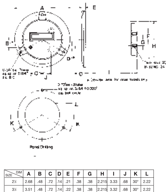
Fig. 23. 2 1/2-3 1/2-inch Type 240 round case
