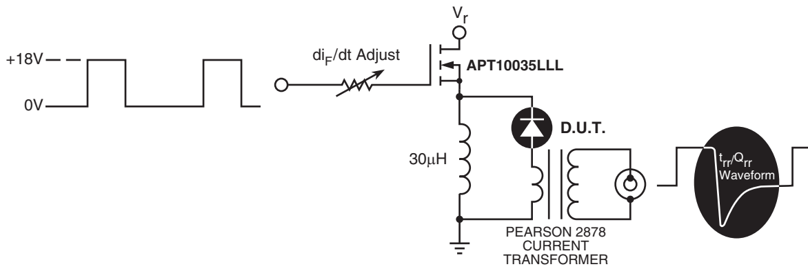
Figure 12, Diode Test Circuit
