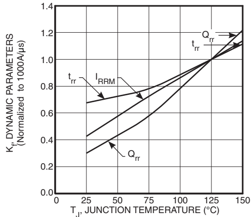
Figure 9. Dynamic Parameters vs. Junction Temperature
