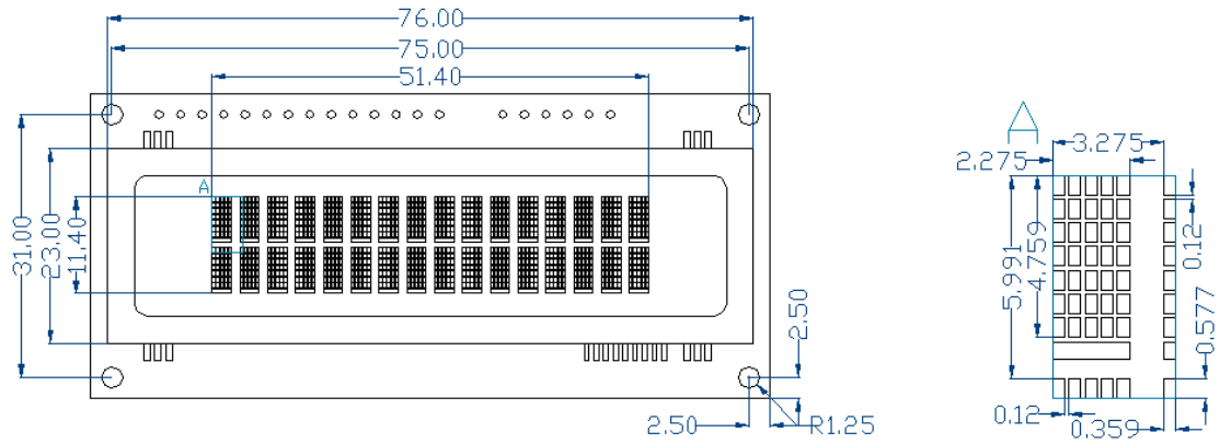
Figure 22: VK162-12 Dimensional Drawing
