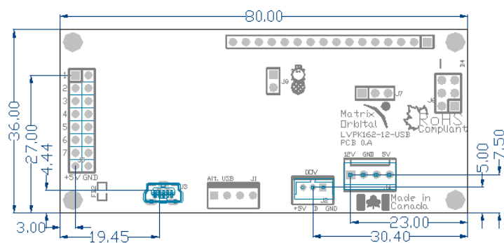
Figure 21: LK162-12-USB Dimensional Drawing
