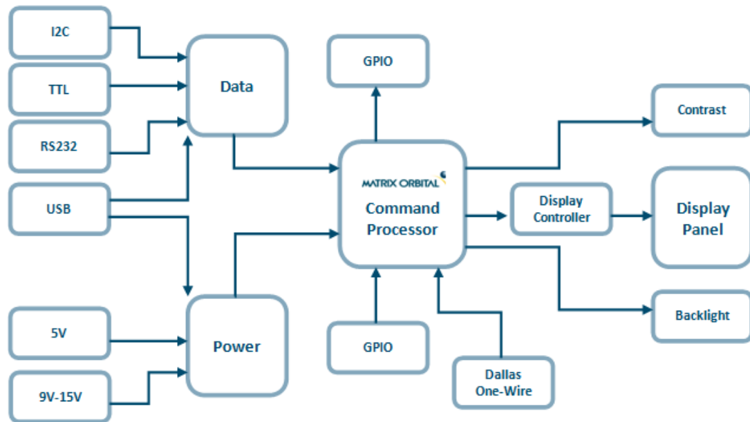
Figure 18: Functional Diagram
