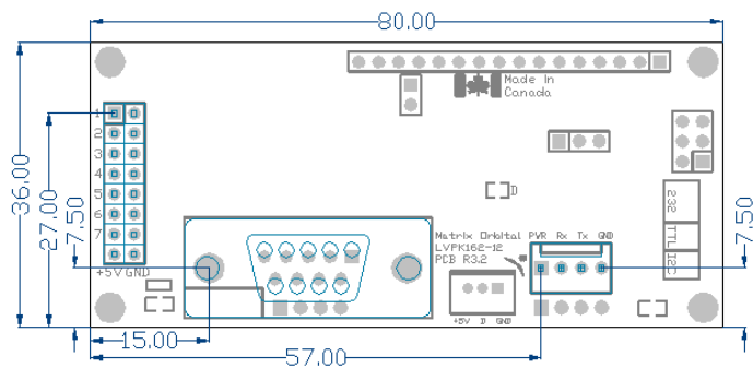
Figure 20: LK162-12 Dimensional Drawing
