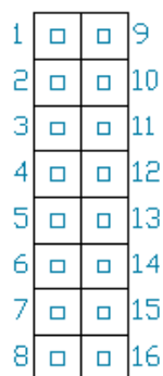
Figure 14: GPIO Header
