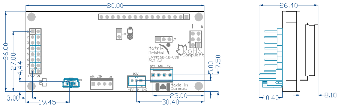
Figure 24: VK162-12 Dimensional Drawing
