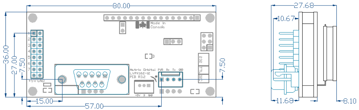
Figure 23: VK162-12 Dimensional Drawing
