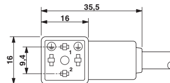
Dimensioned drawing
