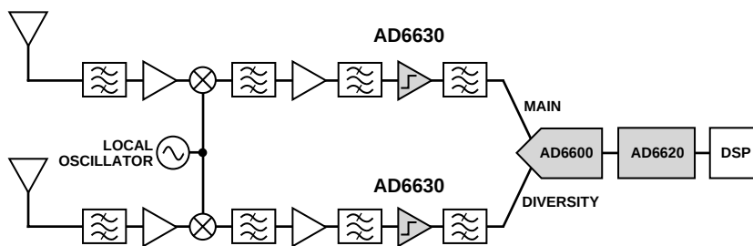
Figure 1. Reference Design
