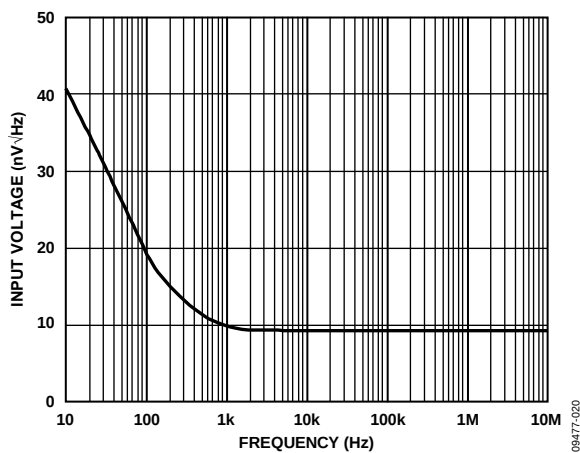
Figure 20. Input Voltage vs. Frequency
