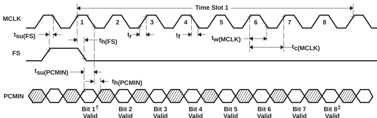
Figure 3. PCM Transmit Timing
