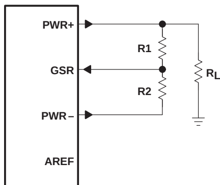
Figure 13. Single-Ended Configuration
