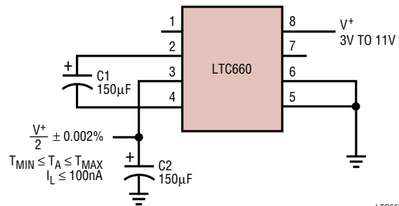
Figure 9. Ultraprecision Voltage Divider
