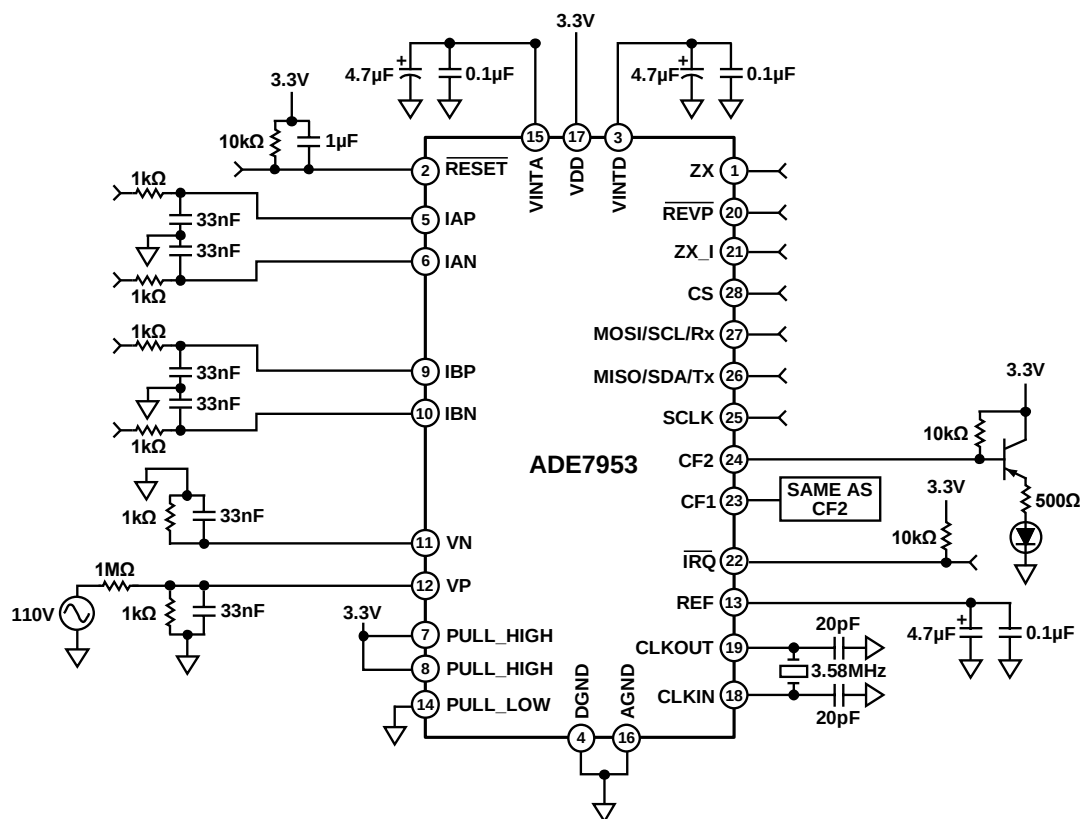
Figure 35. Test Circuit
