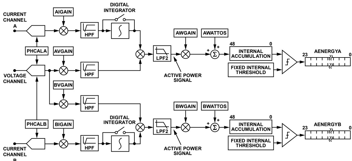
Figure 45. Active Energy Signal Chain
