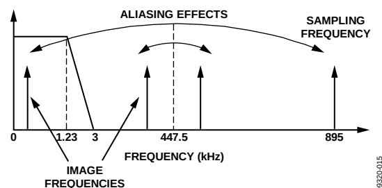
Figure 38. Aliasing Effect
