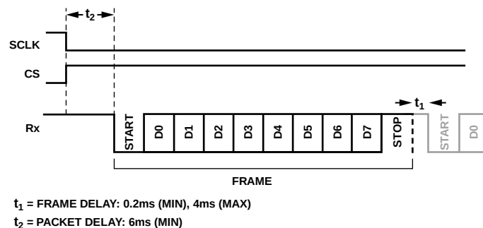
Figure 72. UART Frame
