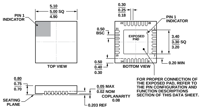
Figure 79. 28-Lead Lead Frame Chip Scale Package [LFCSP_WQ] 5 mm x 5 mm Body, Very Very Thin Quad (CP-28-6) Dimensions shown in millimeters
