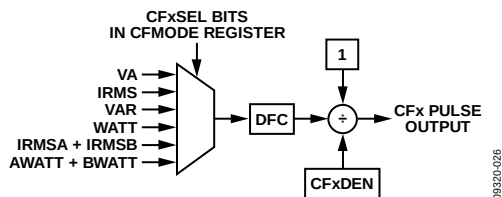
Figure 57. Energy-to-Frequency Conversion
