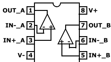
ISL28233IUZ (8 LD MSOP) TOP VIEW
