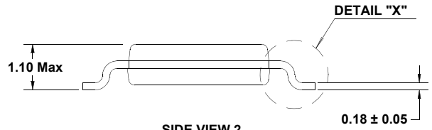
SIDE VIEW 2
