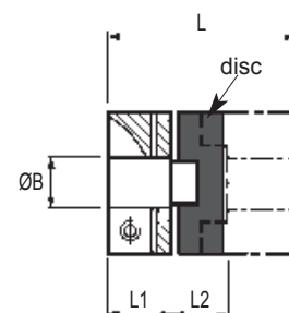
Refs. 452, 453, 456 Clamp style
