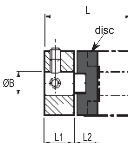
Refs. 450, 454 Set screw style
