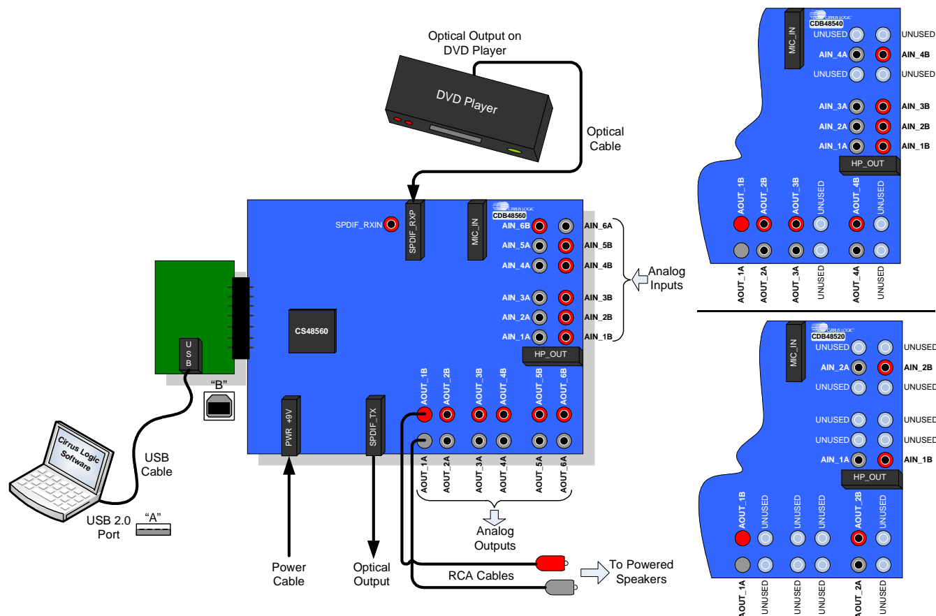
Figure 2-2. Board Setup Diagram
