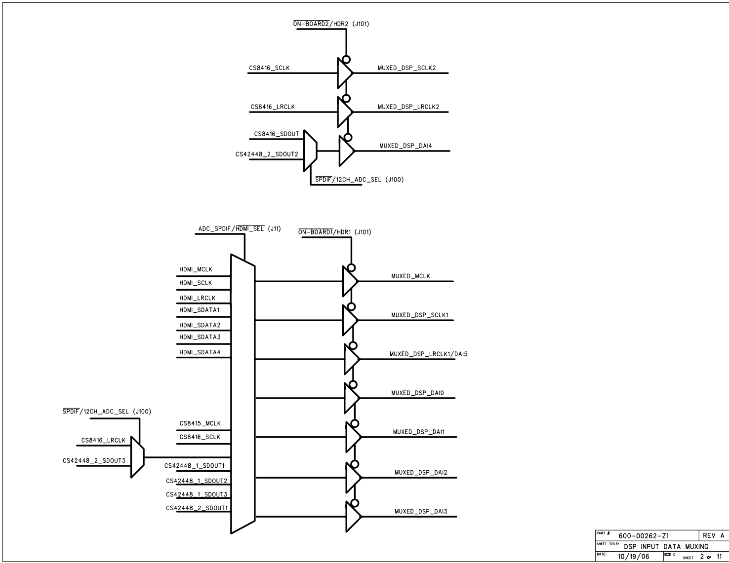
Figure A-2. DSP Input Data Multiplexing Schematic
