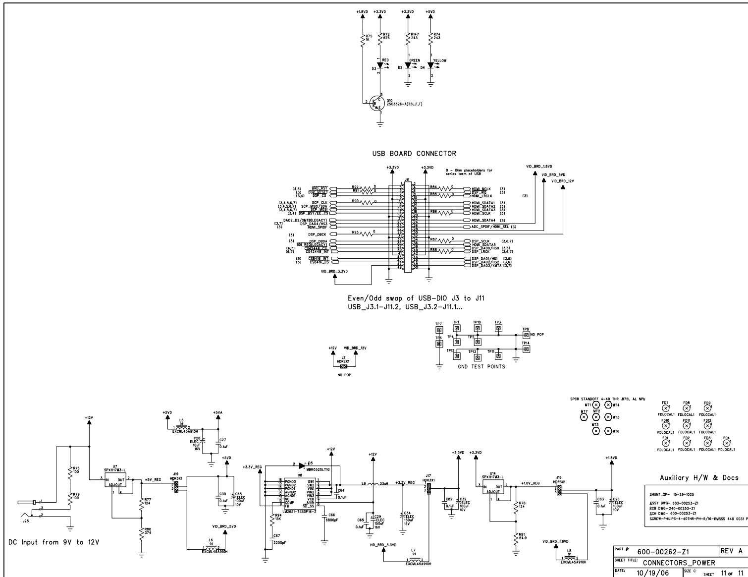
Figure A-11. Control Connector and Power Schematic
