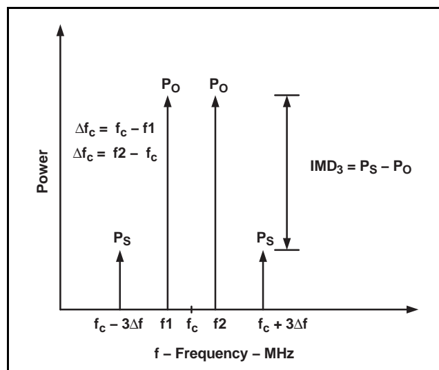
Figure 107. 2-Tone and 3rd-Order Intermodulation Products
