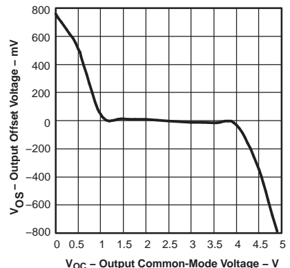
OUTPUT OFFSET VOLTAGE vs OUTPUT COMMON-MODE VOLTAGE
