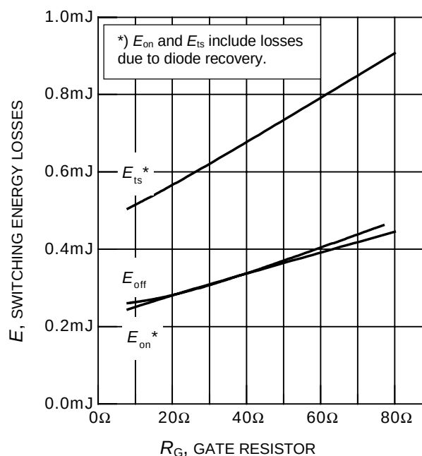
Figure 14. Typical switching energy losses as a function of gate resistor (inductive load, T_j = 150^\circ\text{C} , V_{CE} = 400\text{V} , V_{GE} = 0/+15\text{V} , I_C = 10\text{A} )
