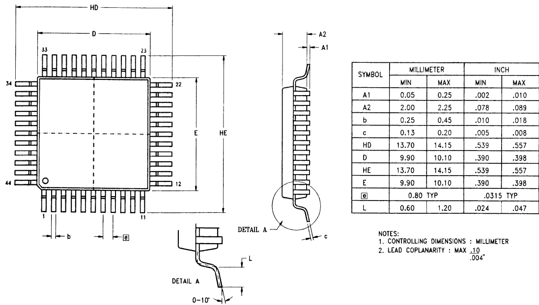
Figure 27. 44-Pin QFP Package Diagram
