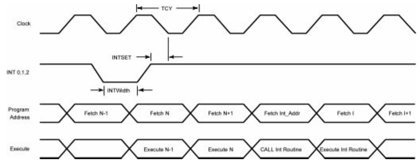
Figure 11. Interrupt Timing
