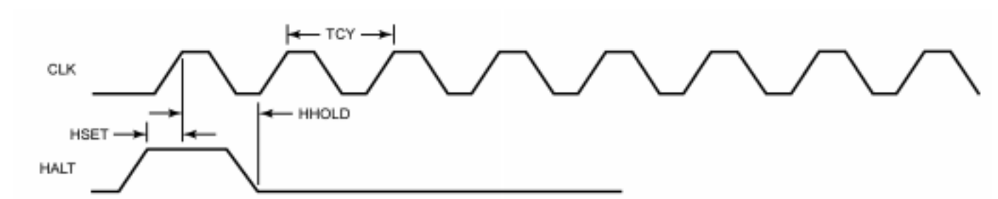
Figure 12. HALT Timing
