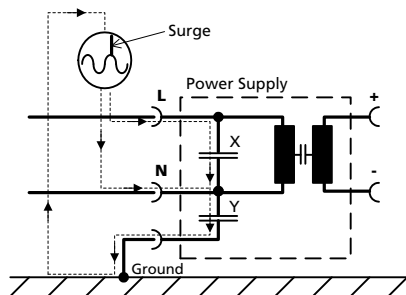
Fig. 23-3 Earthed input
