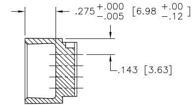
SECTION X-X
