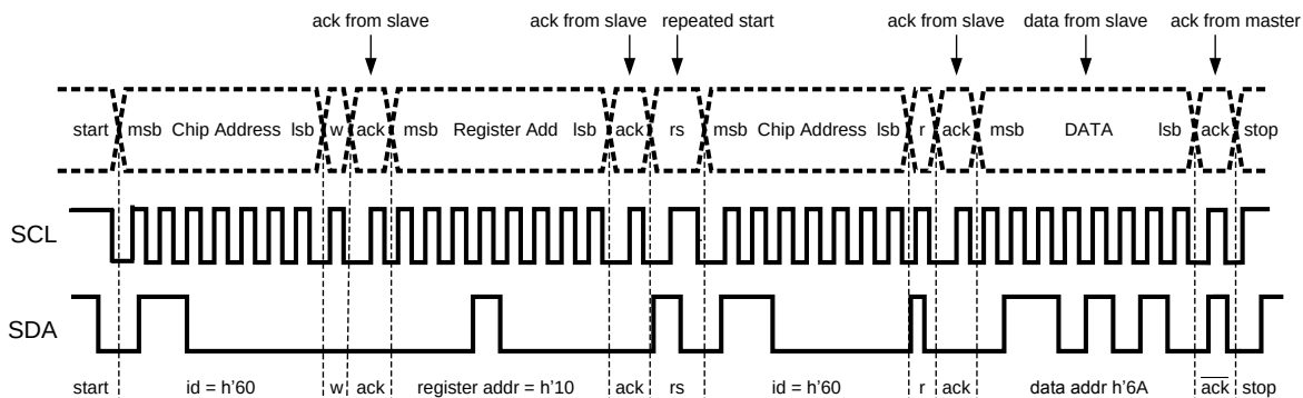
Figure 38. I²C Read Cycle
