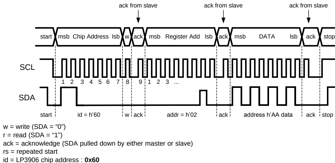
Figure 37. I²C Write Cycle
