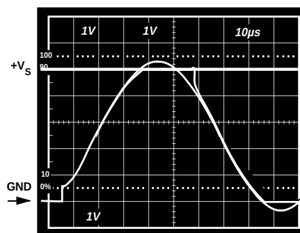
b. V_{IN} = 0 to +V_S + 200 mV; V_{OUT} = 0 to +V_S ; R_P = 49.9 k \Omega
