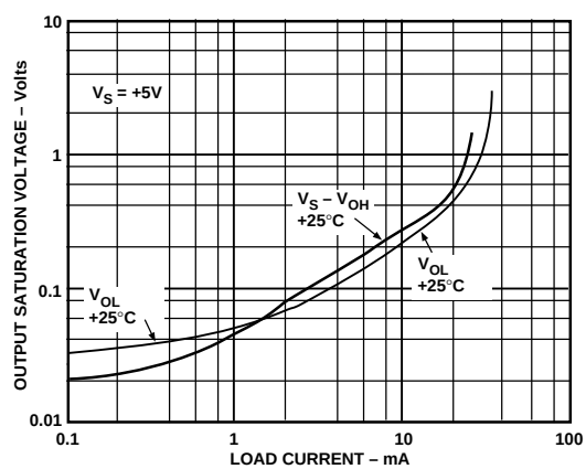
Figure 20. Output Saturation Voltage vs. Load Current
