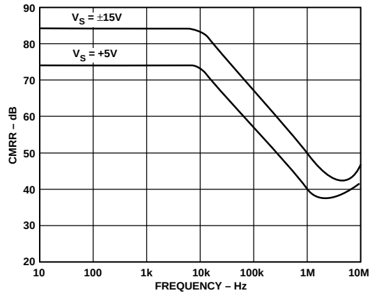
Figure 19. Common-Mode Rejection vs. Frequency
