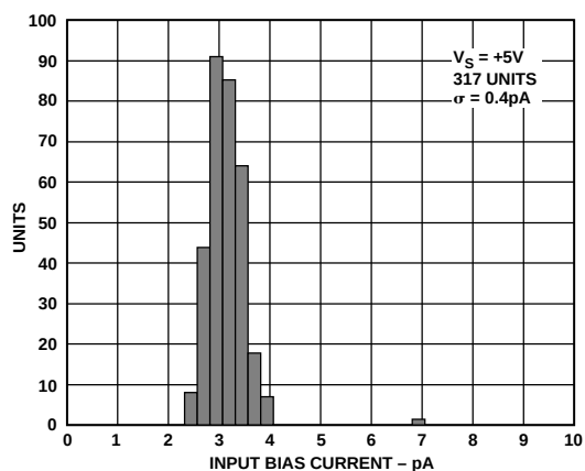
Figure 7. Typical Distribution of Input Bias Current
