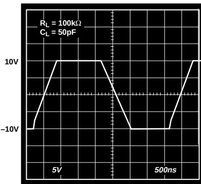
Figure 34. Pulse Response, V_S = \pm 15\text{ V} , G = +1
