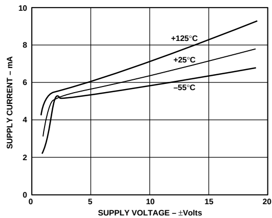
Figure 21. Quiescent Current vs. Supply Voltage
