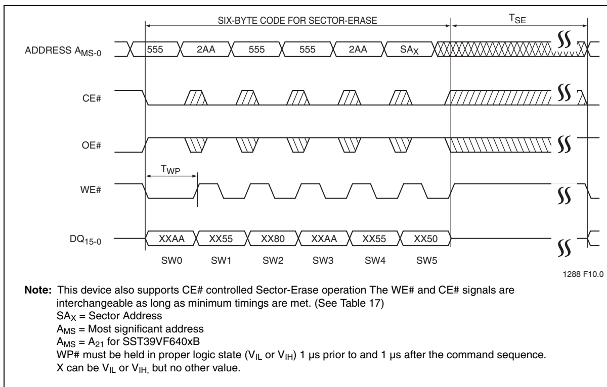
Figure 10: WE# Controlled Sector-Erase Timing Diagram
