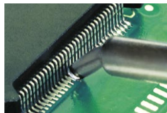
SMD soldering with the Micro tool
