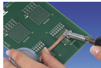
Removal of residual solder
