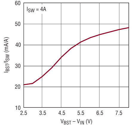
Boost Drive vs Boost Voltage
