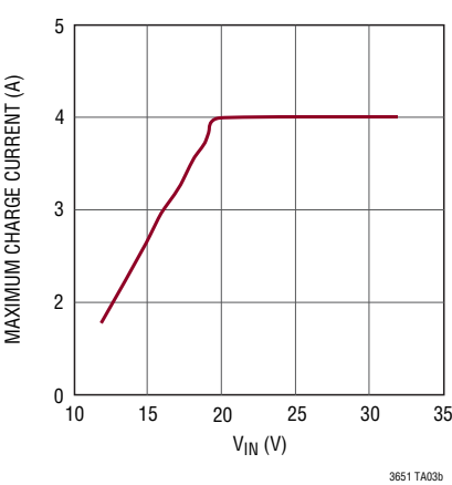
Maximum Charge Current vs VIN
