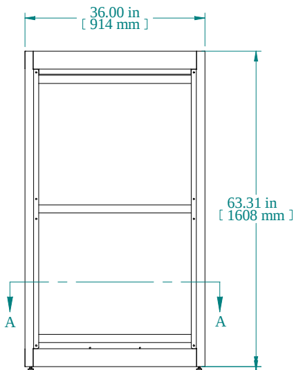
L.S. VIEW
