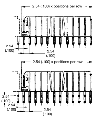
Recommended PCB layouts
