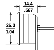
Backlit Bezel Mount Side View
