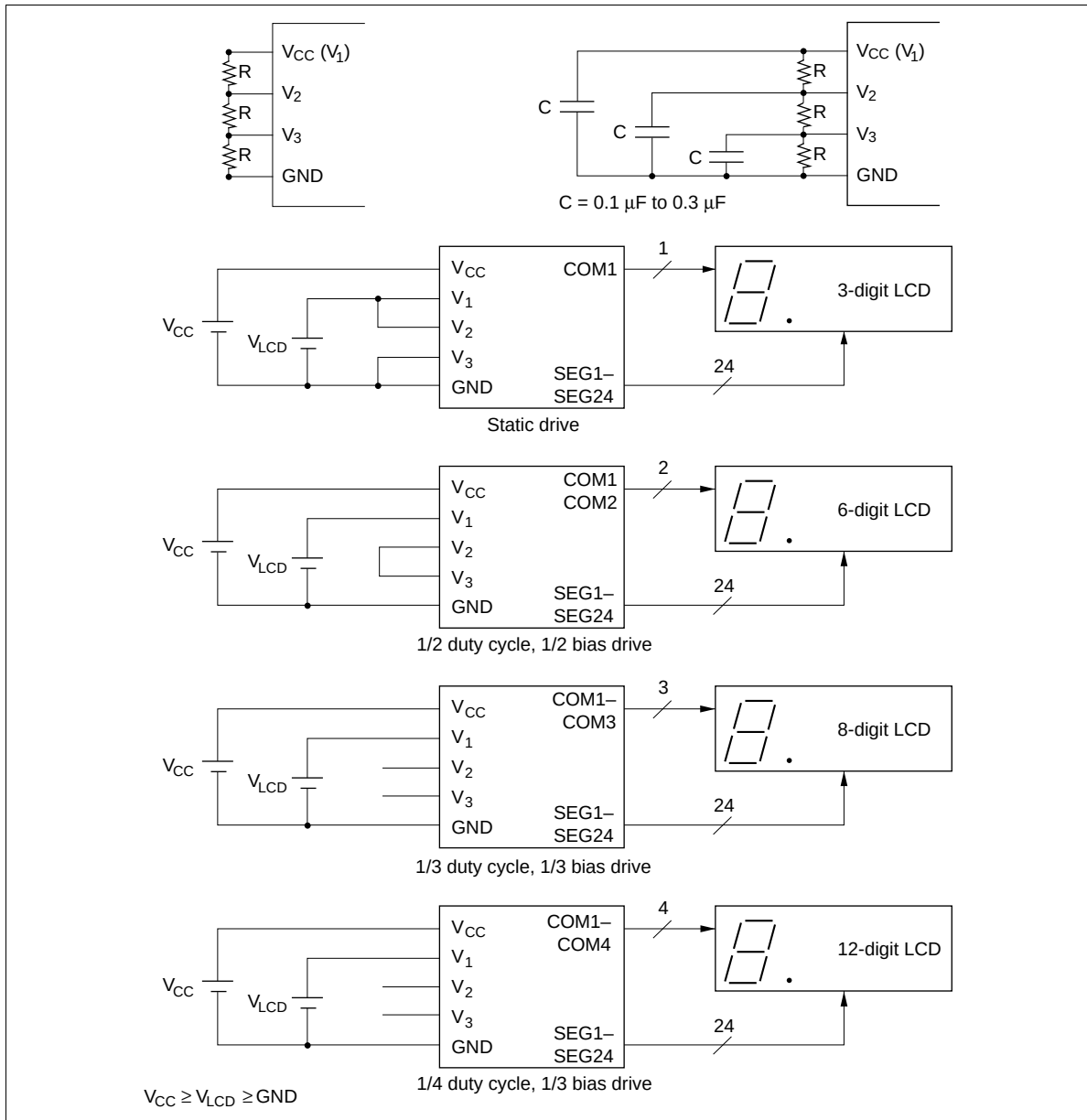
Figure 40 LCD Connection Examples
