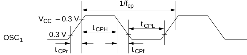
Figure 49 Oscillator Timing
