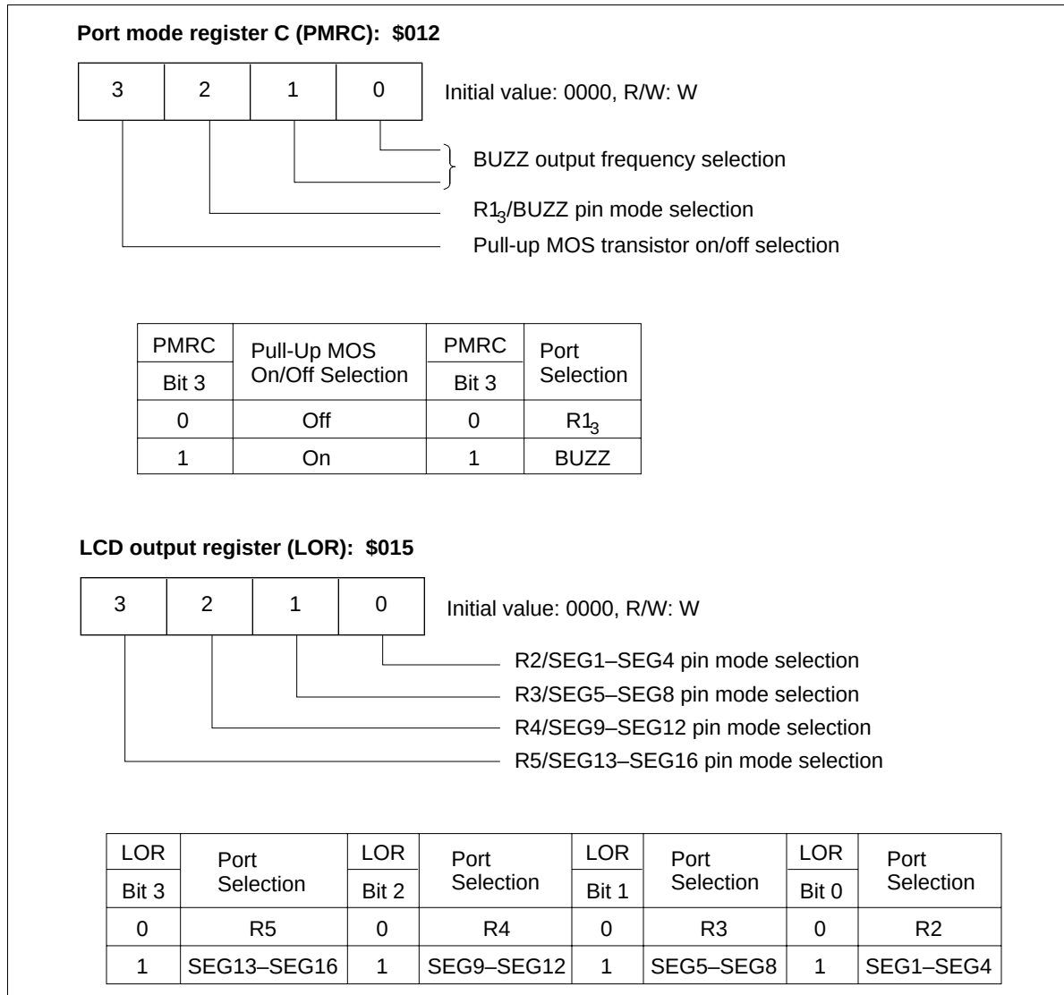
Figure 24 I/O Switching Mode Registers (cont)
