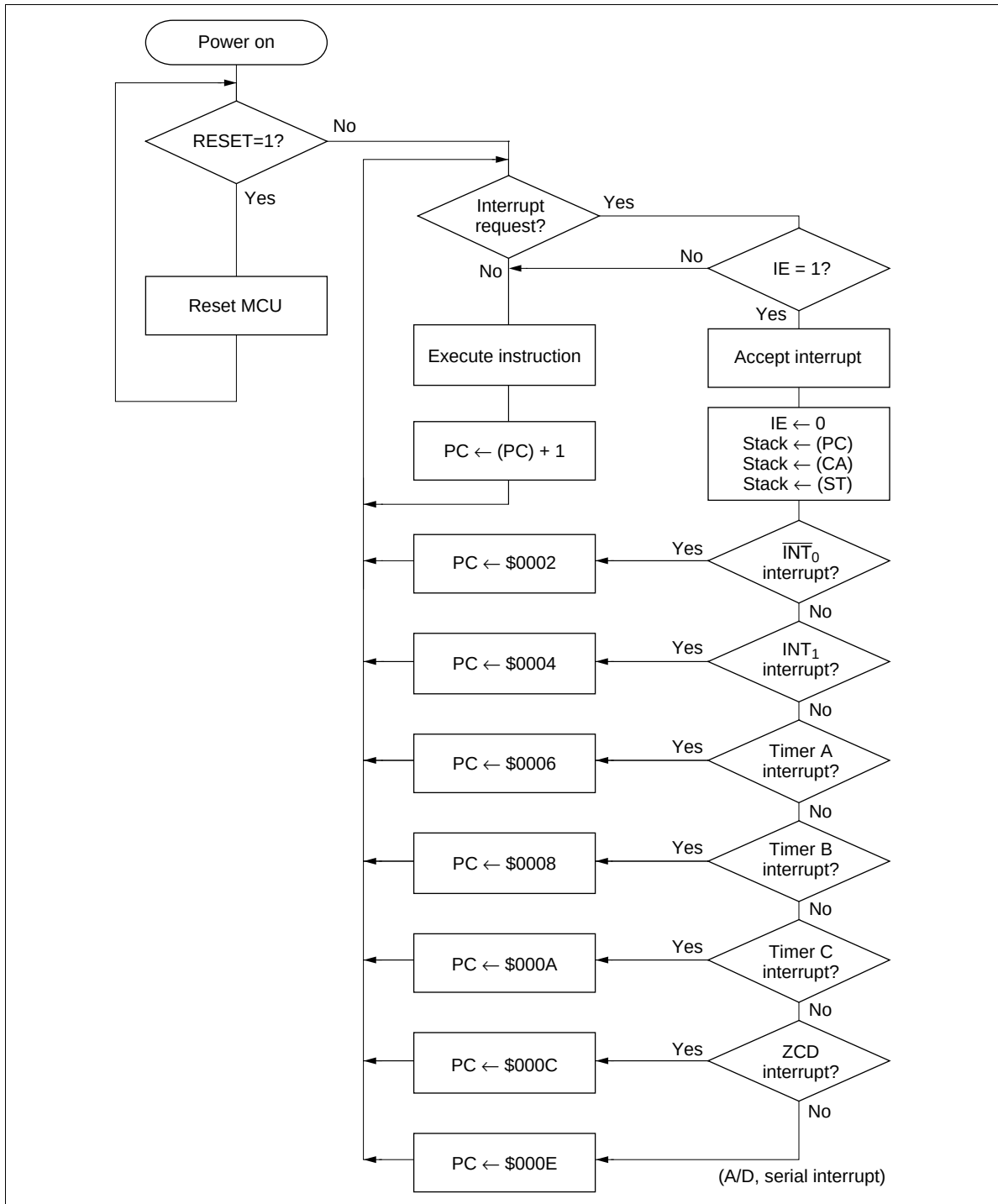
Figure 8 Interrupt Processing Flowchart
