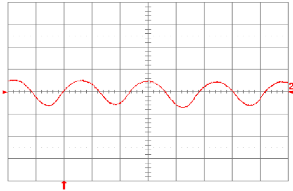
Fig. 8.0V.15: Input reflected ripple current, i_c (100 mA/div.), measured at input terminals at full rated load current and V_{in} = 48V . Refer to Fig. 8.0V.14 for test setup. Time scale: 1 \mu s /div.
