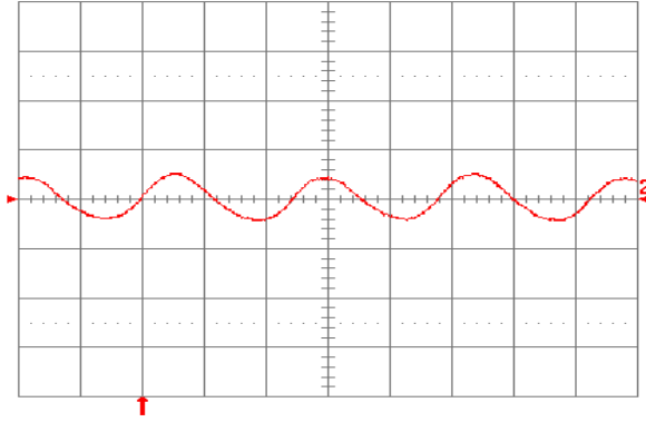
Fig. 3.3V.15: Input reflected ripple current, i_c (100 mA/div.), measured at input terminals at full rated load current and V_{in} = 48 V. Refer to Fig. 3.3V.14 for test setup. Time scale: 1 \mu s/div.
