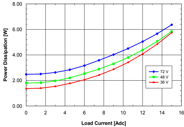
Fig. 2.5V.7: Power dissipation vs. load current and input voltage for SQ48T/S15025 converter mounted vertically with air flowing from pin 3 to pin 1 at a rate of 300 LFM (1.5 m/s) and T_a = 25^\circ\text{C} .
