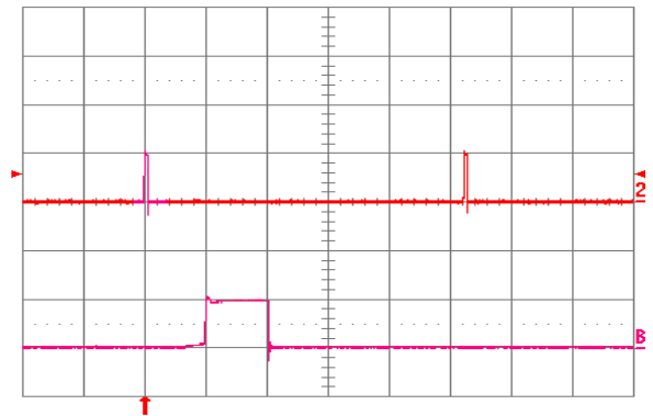
Fig. 1.5V.18: Load current (top trace, 20 A/div., 20 ms/div.) into a 10 m \Omega short circuit during restart, at V_{in} = 48 V. Bottom trace (20 A/div., 1 ms/div.) is an expansion of the on-time portion of the top trace.
