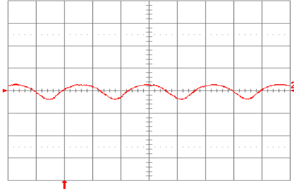
Fig. 1.2V.15: Input reflected ripple current, i_c (100 mA/div.), measured at input terminals at full rated load current and V_{in} = 48 V. Refer to Fig. 1.2V.14 for test setup. Time scale: 1 \mu s/div.
