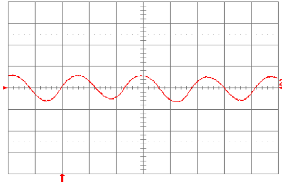
Fig. 5.0V.15: Input reflected ripple current, i_c (100 mA/div.), measured at input terminals at full rated load current and V_{in} = 48V . Refer to Fig. 5.0V.14 for test setup. Time scale: 1 \mu s /div.
