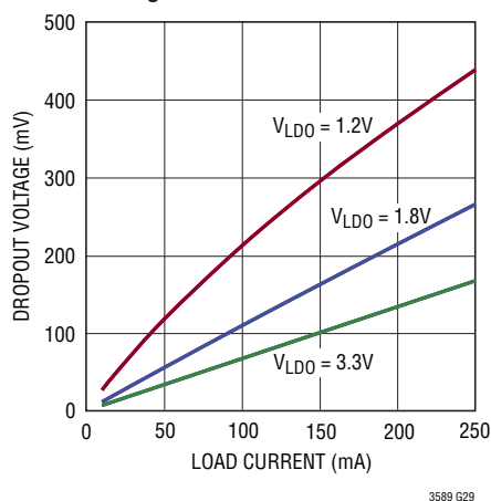
LD02, LD03, LD04 Dropout Voltage vs Load Current
