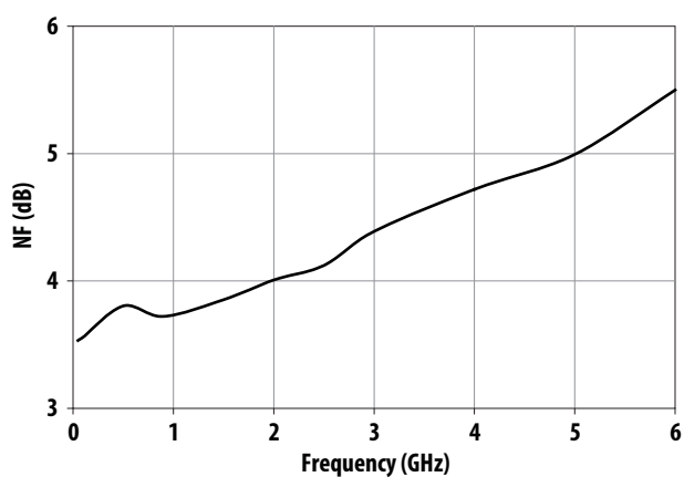
Figure 8. NF vs Frequency at I_d = 36\text{mA}
