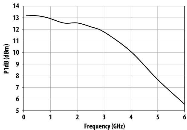
Figure 6. P1dB vs Frequency at I_d = 36\text{mA}
