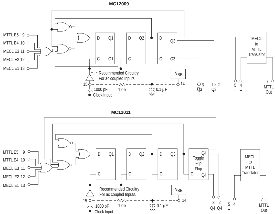
Figure 1. Logic Diagrams
