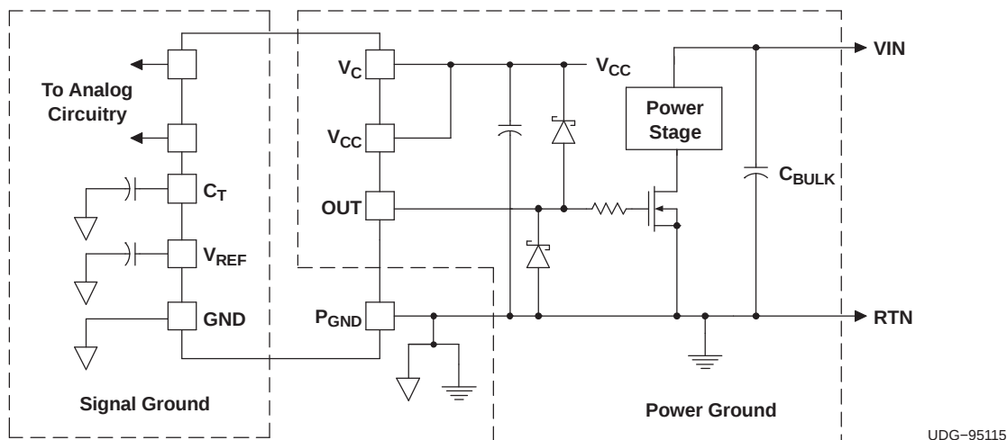
Figure 13. Ground Planes
