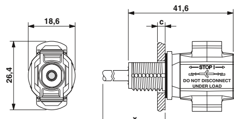
Dimension: pin (-), dimension x = cable length
