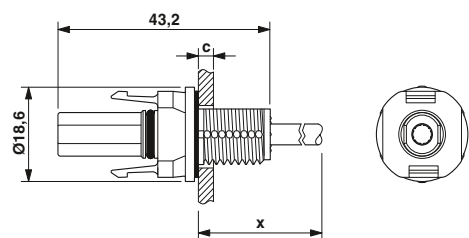
Dimension: socket (+), dimension x = cable length
