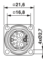
Flange dimensions 21.6 mm x 21.6 mm
