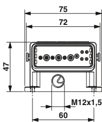
Dimensional drawing: panel mounting base
