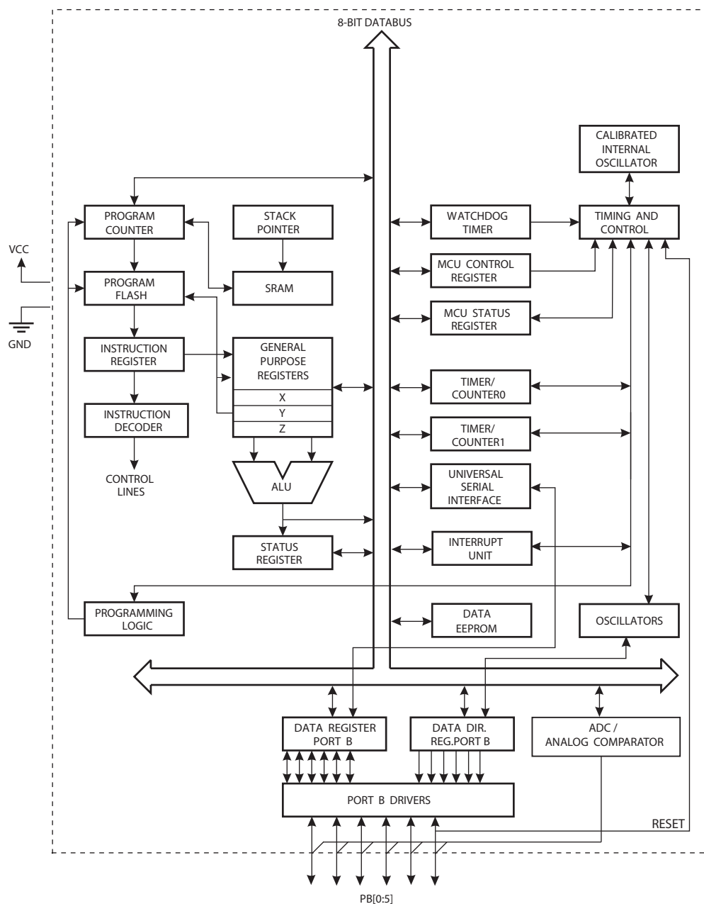
Figure 2-1. Block Diagram
