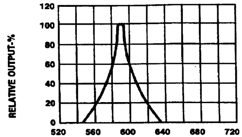
Fig.2 SPECTRAL RESPONSE
