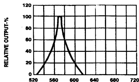
Fig.2 SPECTRAL RESPONSE
