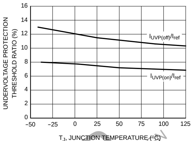
Figure 14. Undervoltage Protection Thresholds vs. Temperature
