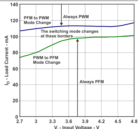
Figure 40. PFM/PWM Boundaries
