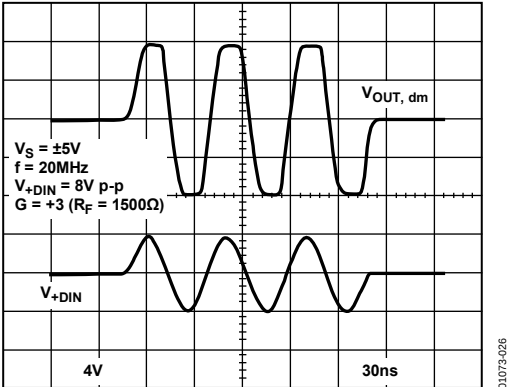
Figure 26. Output Overdrive
