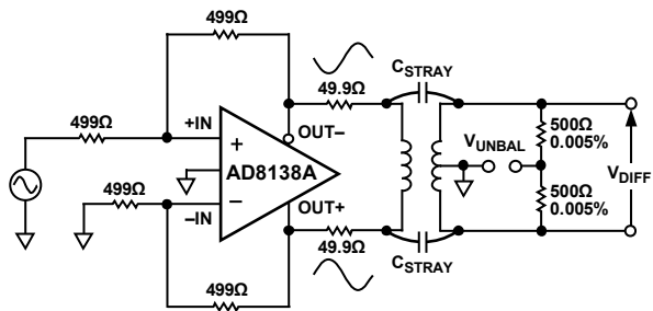
Figure 44. AD8138A Forms a Balanced Transformer Driver
