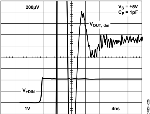
Figure 25. Settling Time
