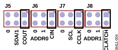
Figure 4. SPI Control
