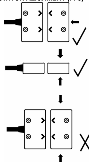
FIGURE 3. SWITCH ALIGNMENT (FF5)
