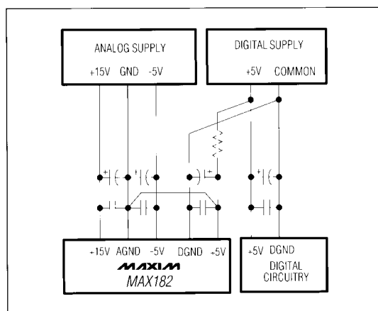
Figure 16. Power-Supply Grounding
