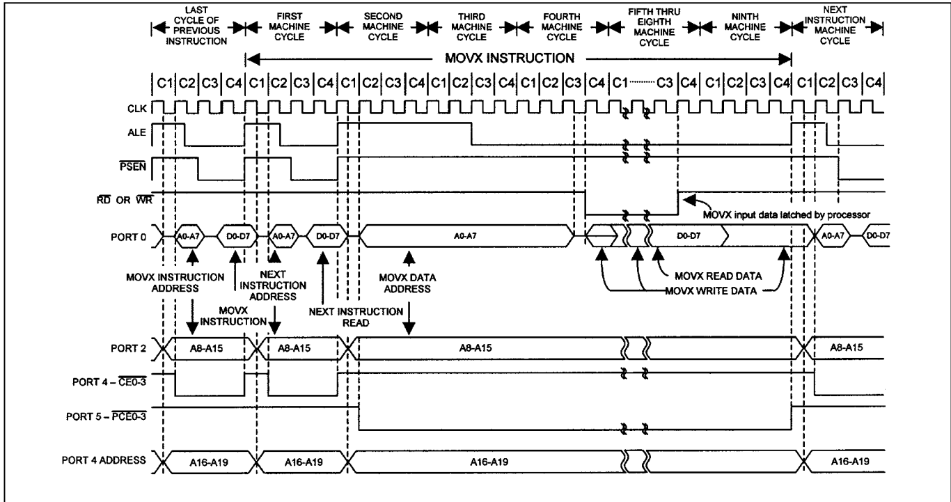
Figure 10. Multiplexed 9-Cycle Data Memory \overline{PCE0-3} Read or Write
